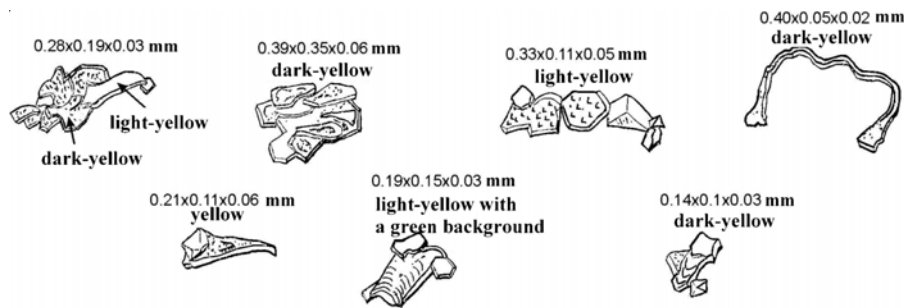
Figure 2: Forms of native gold plates discovered in the channel deposits in the Canyon Makhtesh Ramon (northern Negev), (prepared by A.V. Surkov).
