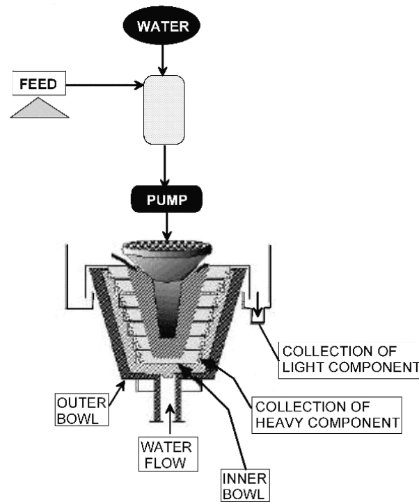
Figure 1: Centrifugal gravity separator: a simplified scheme.
