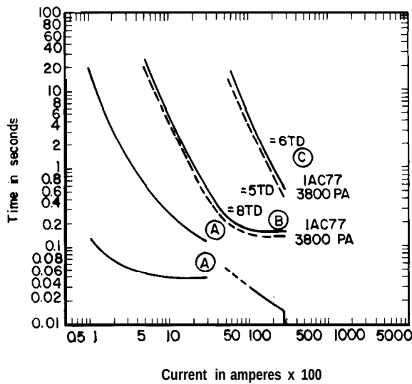
Fig. 24. Pole-type recloser vs IAC 77 relay coordination example
