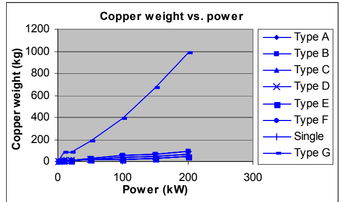
Fig. 17 Copper weight vs. power for high-speed machines
