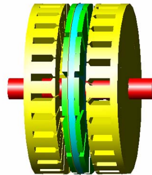
Fig.3 Axial-flux construction with double stators
