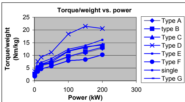
Fig.11 torque per weight vs power for direct-driven machines
