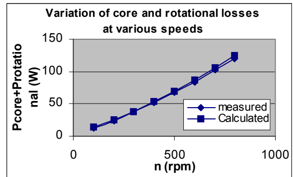
Fig. 9 Variation of core and rotational losses with speed
