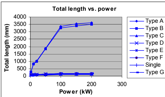
Fig.27 Total length vs power for direct-driven machines
