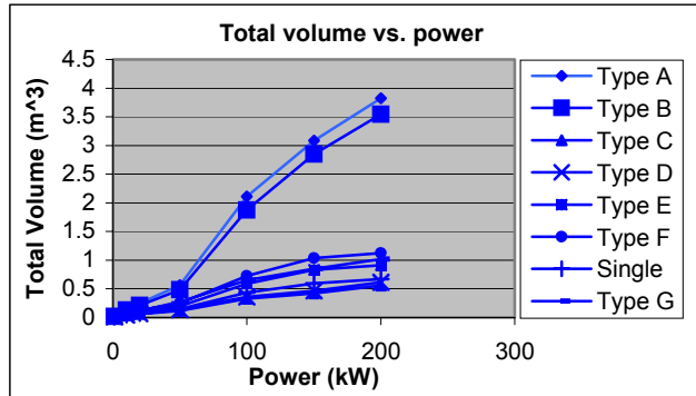
Fig. 20 Total volume vs power for direct-driven machines
