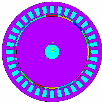
Fig. 1 Inner rotor radial-flux construction
