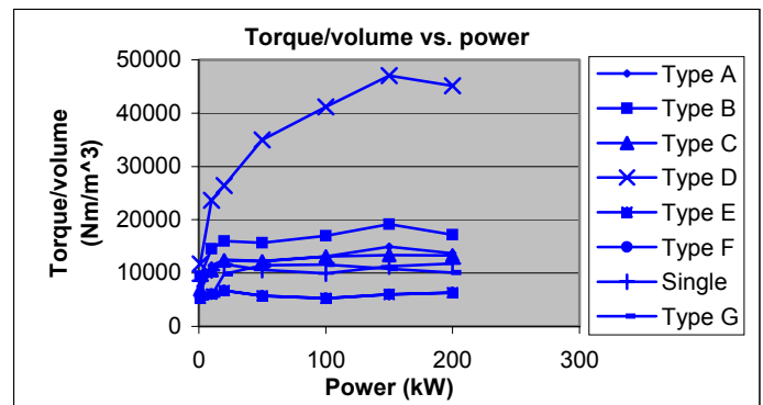
Fig.12 torque per volume vs power for high-speed machines
