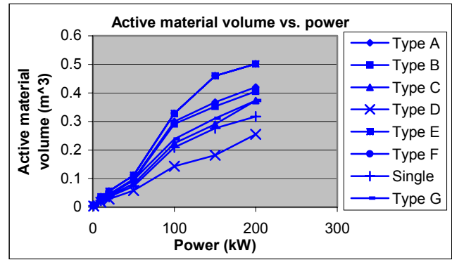
Fig. 22 Active material volume vs power for direct-driven machines
