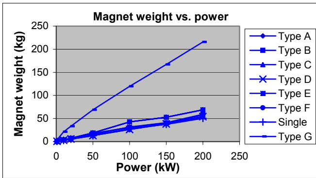
Fig. 15 magnet weight vs. power for high-speed machines
