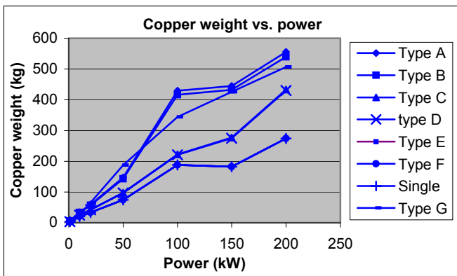
Fig. 16 Copper weight vs. power for direct-driven machines
