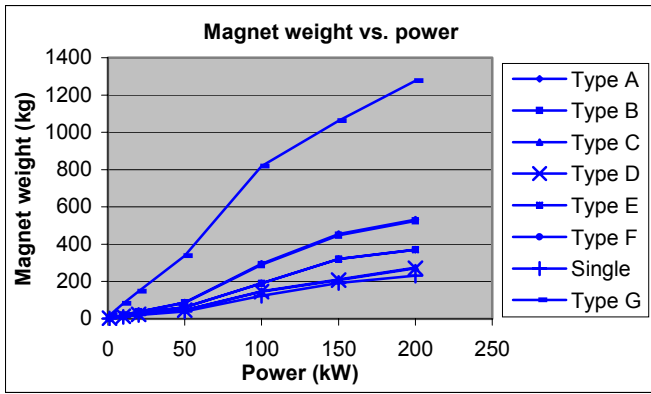
Fig. 14 magnet weight vs. power for direct-driven machines
