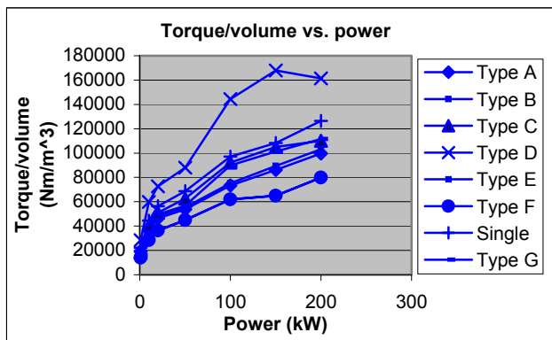
Fig.10 torque per volume vs power for direct-driven machines
