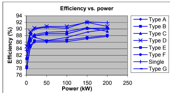
Fig. 24 Efficiency vs power for direct-driven machines
