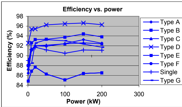
Fig.25 Efficiency vs. power for high speed machines
