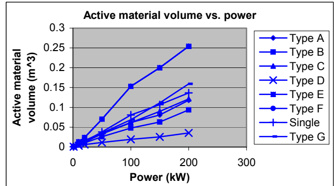
Fig. 23 Active material volume vs power for high-speed machines
