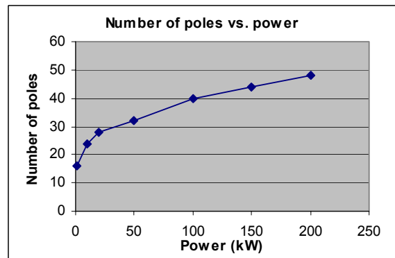
Fig. 6 Number of poles vs. power rating
