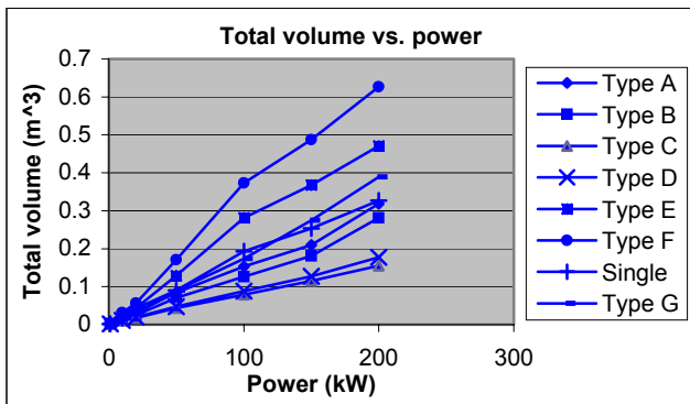
Fig. 21 Total volume vs. power for high-speed machines
