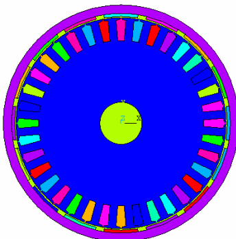
Fig. 2 Radial-flux construction with outer rotor
