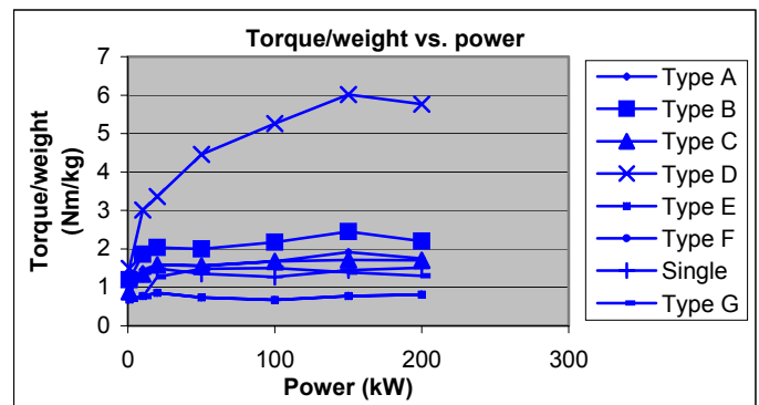
Fig.13 torque per weight vs. power for high-speed machines
