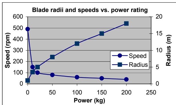
Fig.5 Typical turbine blade radii and rated speed vs. power rating
