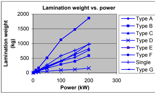
Fig. 19 Lamination weight vs power for high-speed machines
