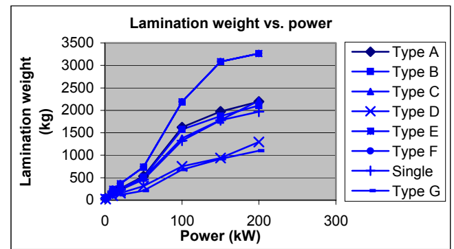
Fig. 18 Lamination weight vs power for direct-driven machines
