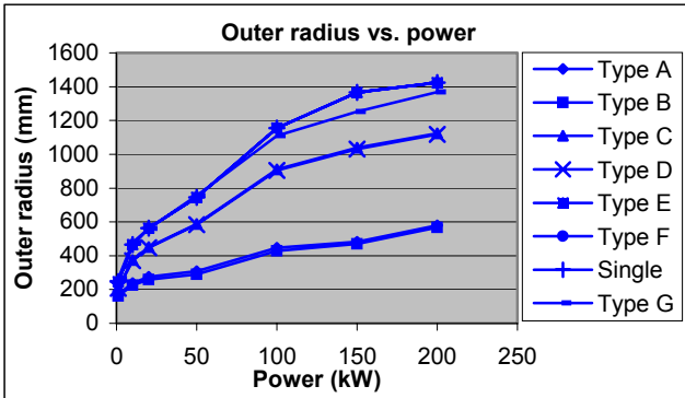
Fig.26 Outer radius vs power for direct-driven machines
