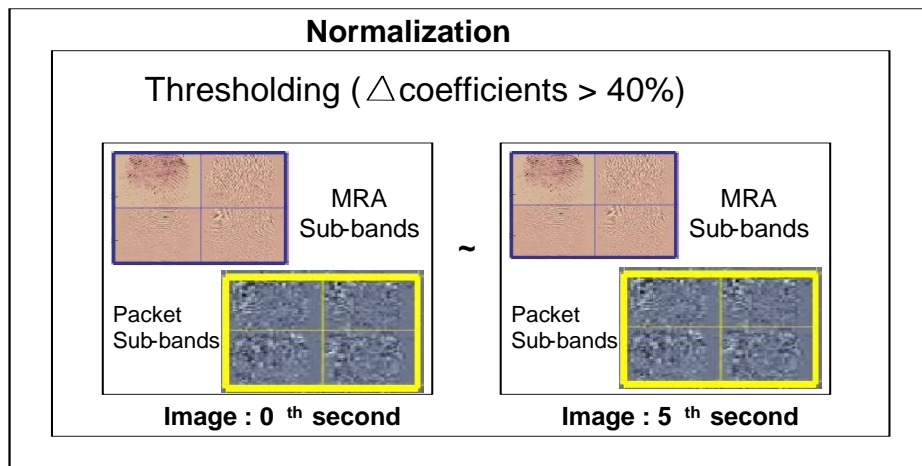
Fig. 2. Algorithm to extract perspiration pattern. Four sub-bands each form Multiresolution analysis and wavelet packets are shown separately.
